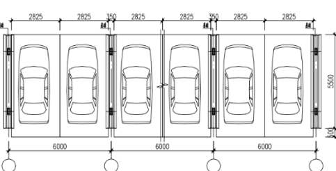
LSC-W8 Foundation
