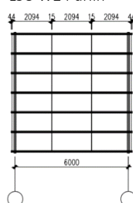
LSC-W6 Purlin
