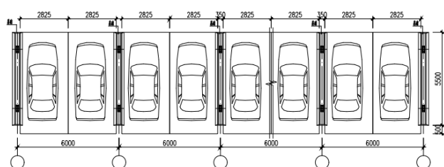
LSC-W10 Foundation
