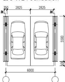
LSC-W6 Foundation
