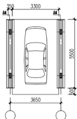
LSC-W2 Foundation
