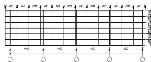
LSC-W10 Purlin
