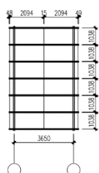
LSC-W2 Purlin
