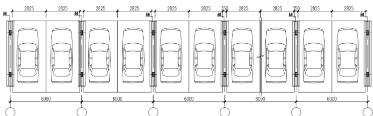
LSC-W10 Foundation
