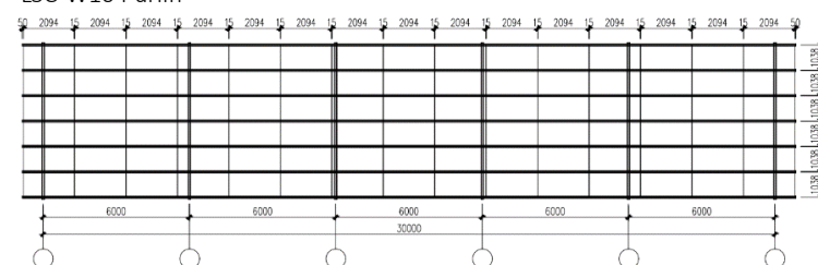
LSC-W10 Purlin
