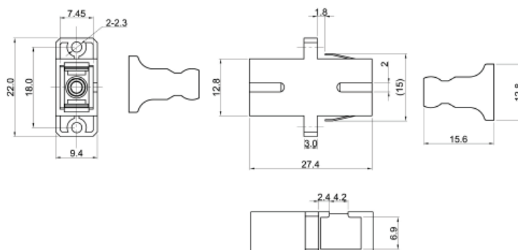
SCAPC-ADAP dimensions in mm
