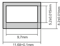
RJ45-6-F-Eco
