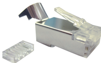
RJ45-6-F
