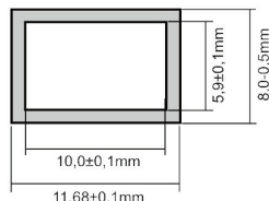
RJ45-6-F
