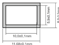
RJ45-6-F
