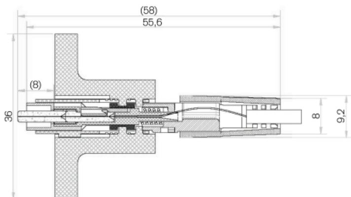
QUICKCON dimensions in mm
