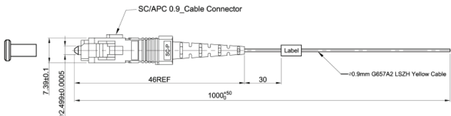
PIGTAIL ICT 1M - dimensions in mm
