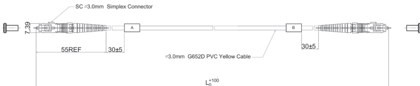
PCFAPC-S series - dimensions in mm
