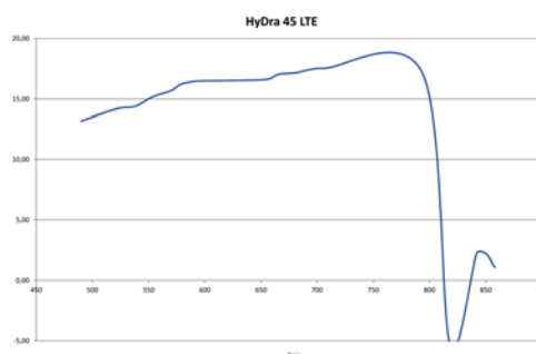
Courbe de gain HyDra 45 Lte
