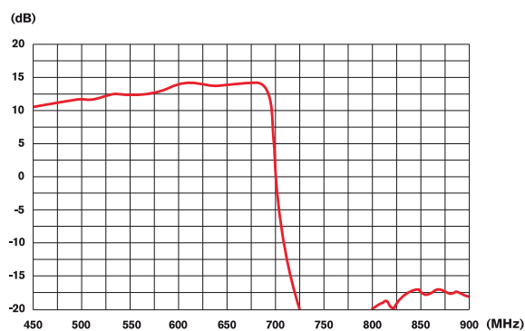
HyDra 35G Gain curve
